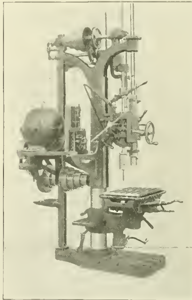
GOULD & EBERHARDT ELECTRICALLY DRIVEN DRILL.
